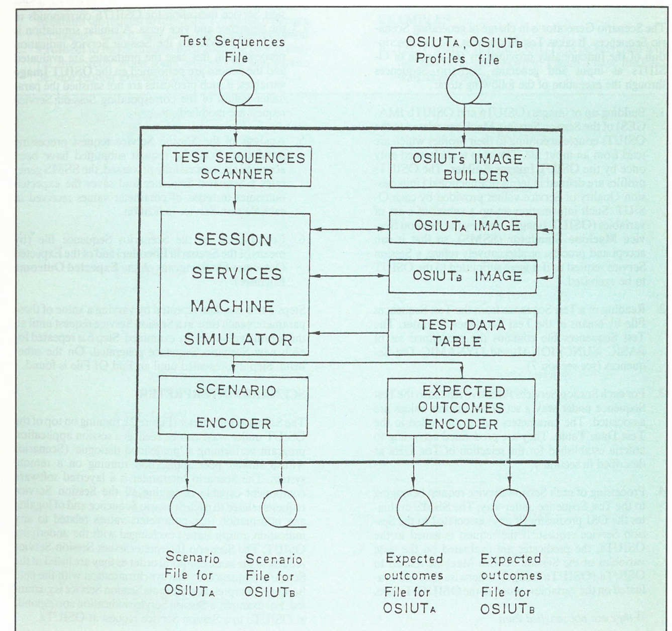
Figure 3 Scenario Generator Structure.
