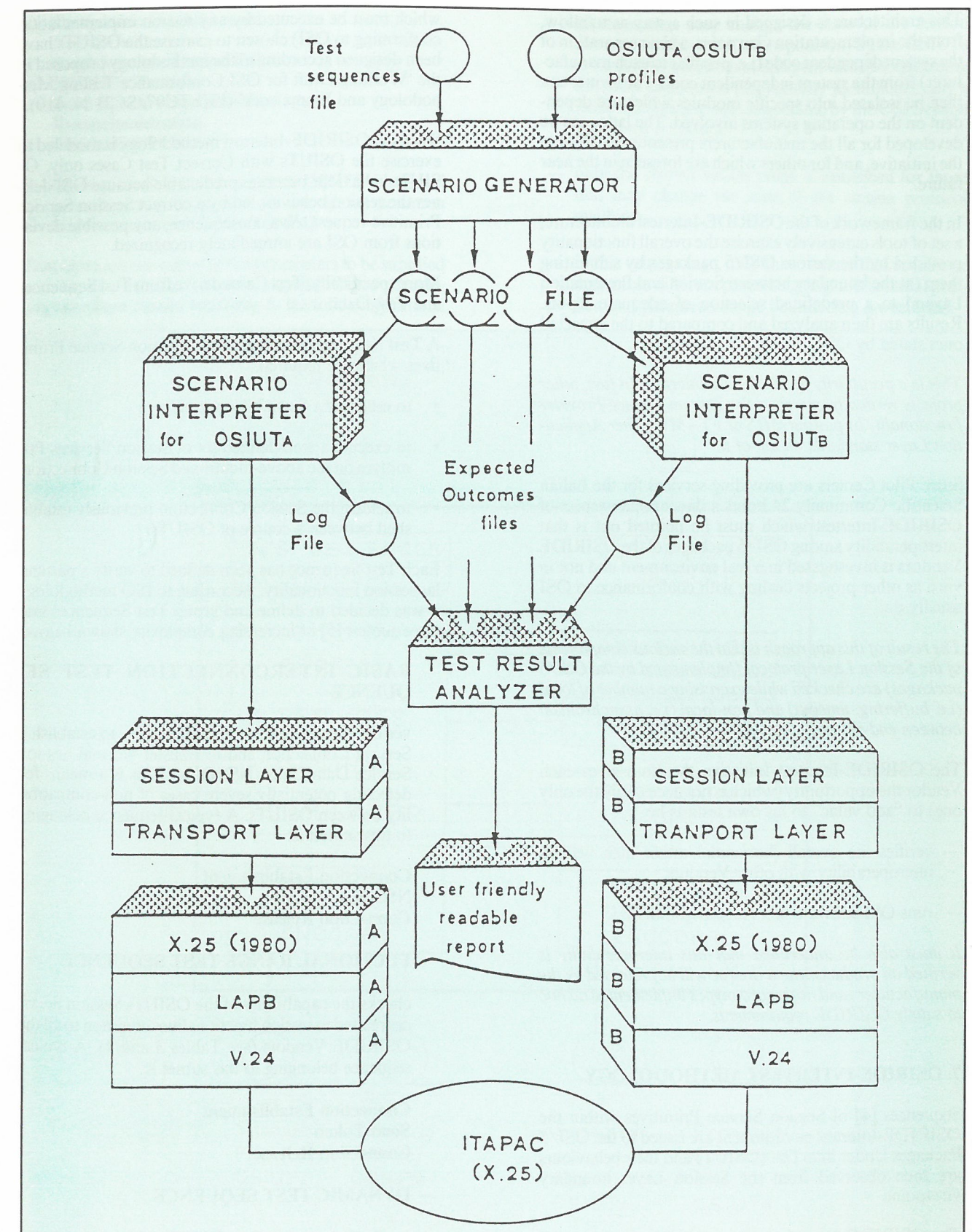
Figure 2 OSIRIDE Interstest architecture.
